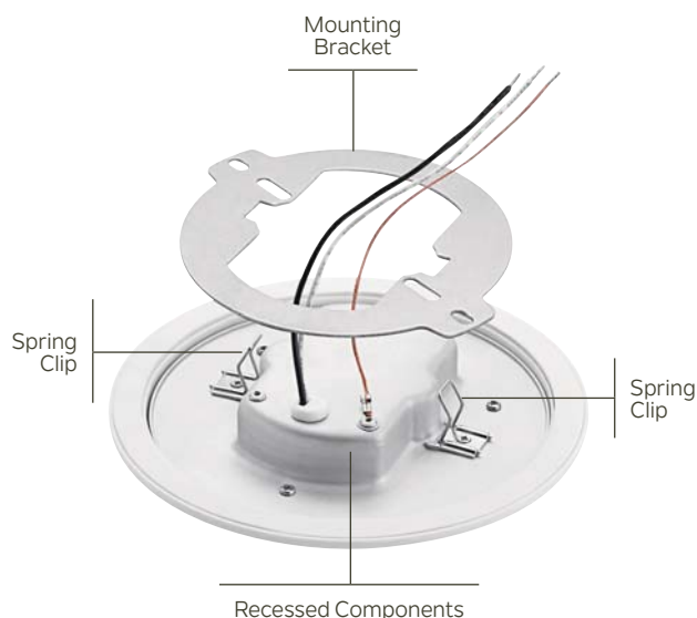
Horizon 43870 Requires 4" x 2-1/8" Round, Square or Octagonal J-Box
